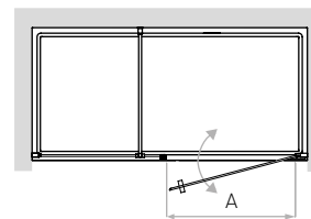
RH Opening
